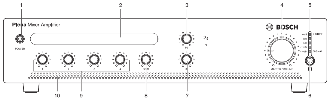
Figure 3.1 Front panel
